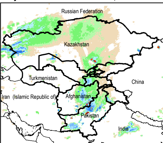
Daily Rainfall estimate for 7 Feb., 2015
