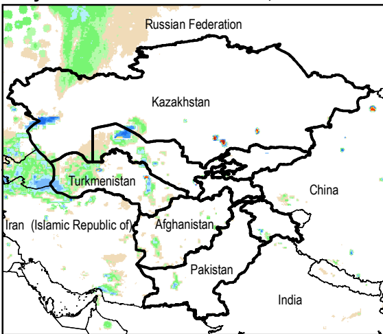
Daily Rainfall estimate for 8 Feb., 2015
