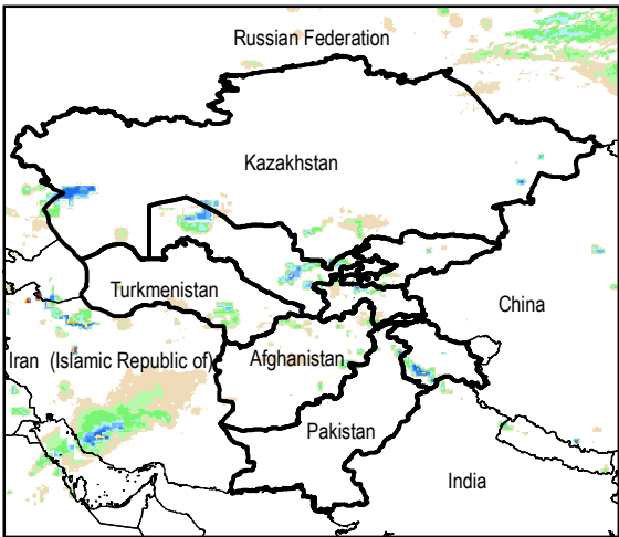
Daily Rainfall estimate for 14 Feb., 2015
