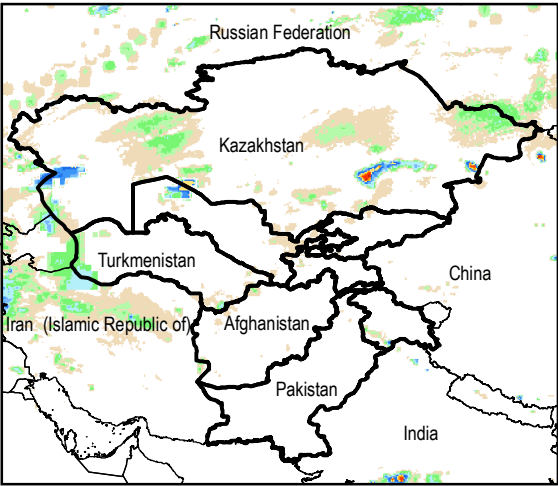
Daily Rainfall estimate for 13 Feb., 2015
