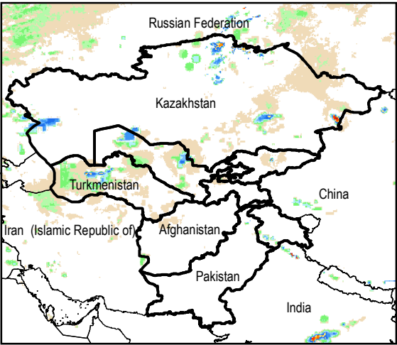
Daily Rainfall estimate for 12 Feb., 2015
