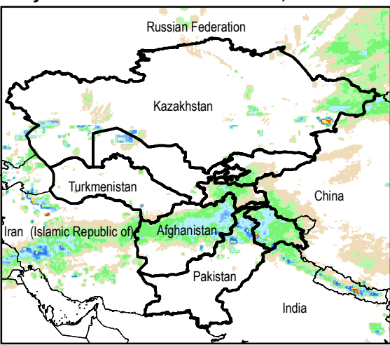
Daily Rainfall estimate for 18 Feb., 2015
