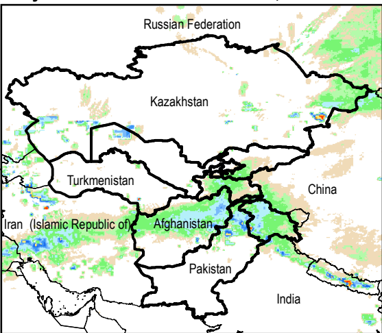
Daily Rainfall estimate for 21 Feb., 2015
