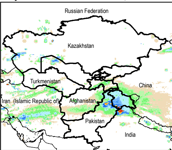
Daily Rainfall estimate for 22 Feb., 2015
