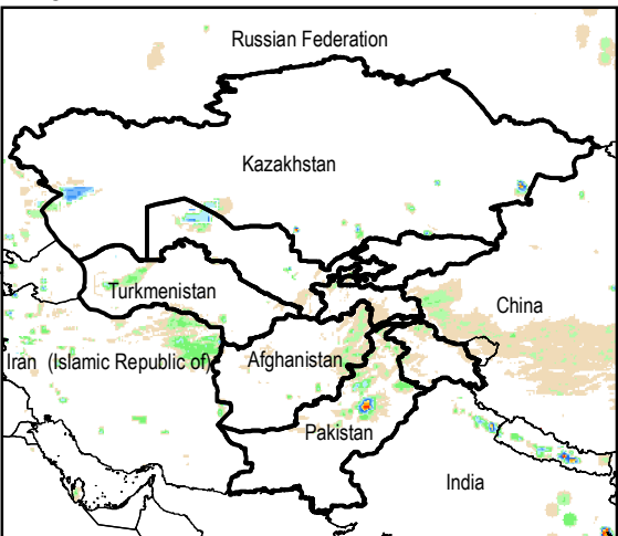
Daily Rainfall estimate for 4 Mar., 2015
