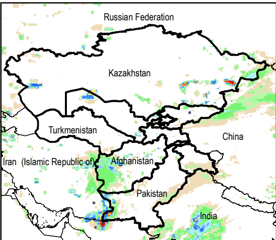
Daily Rainfall estimate for 12 Mar., 2015
