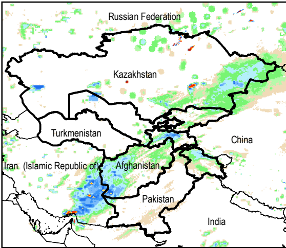
Daily Rainfall estimate for 14 Mar., 2015
