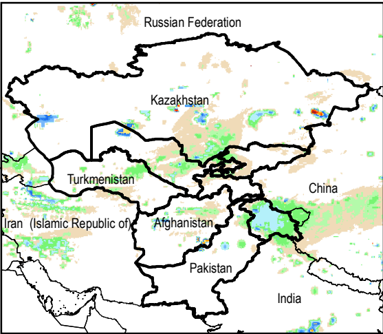
Daily Rainfall estimate for 12 Mar., 2015
