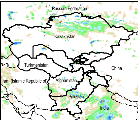
Daily Rainfall estimate for 13 Mar., 2015
