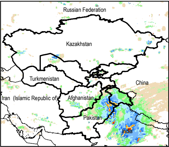
Daily Rainfall estimate for 18 Mar., 2015
