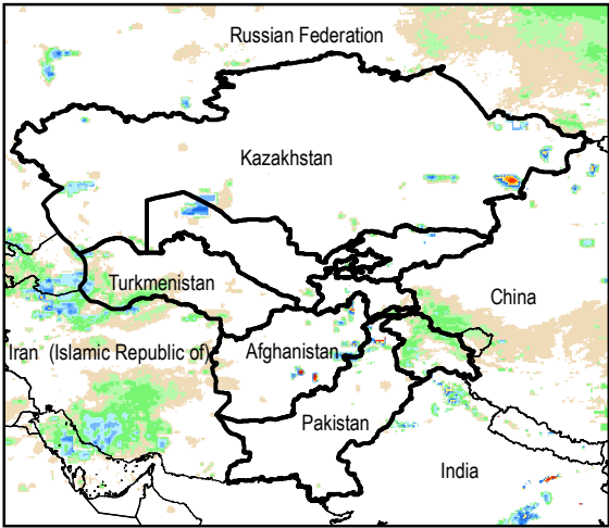
Daily Rainfall estimate for 20 Mar., 2015
