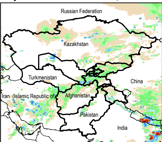
Daily Rainfall estimate for 27 Mar., 2015
