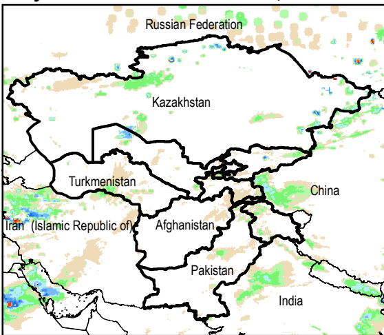
Daily Rainfall estimate for 29 Mar., 2015
