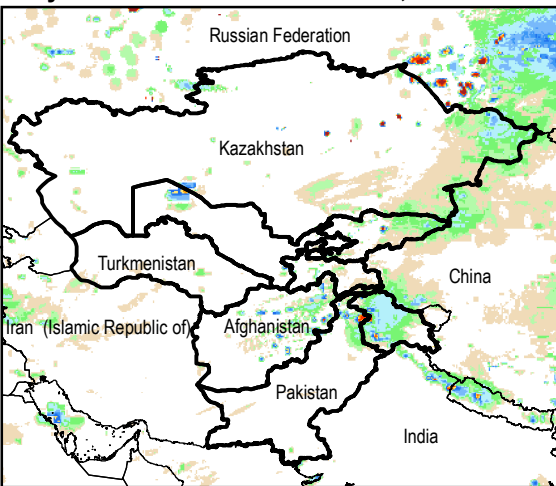
Daily Rainfall estimate for 28 Mar., 2015
