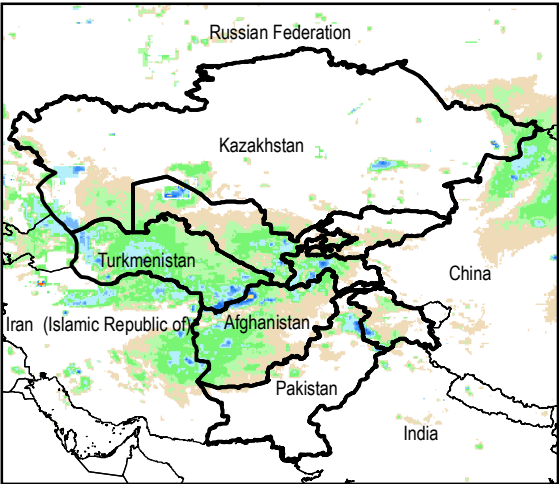
Daily Rainfall estimate for 31 Mar., 2015
