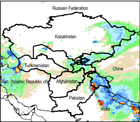
Daily Rainfall estimate for 2 Apr., 2015
