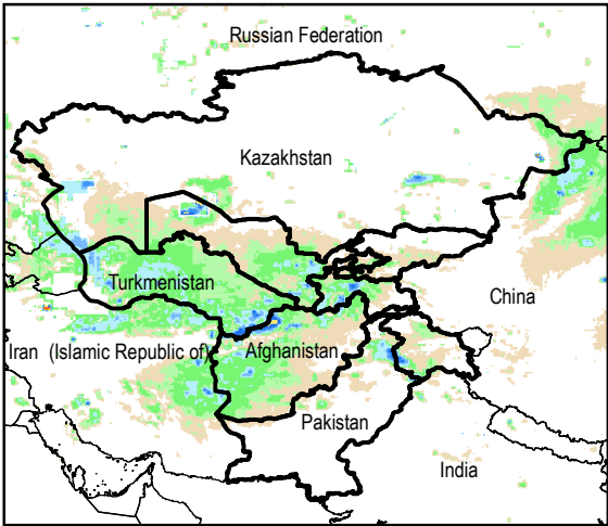
Daily Rainfall estimate for 3 Apr., 2015
