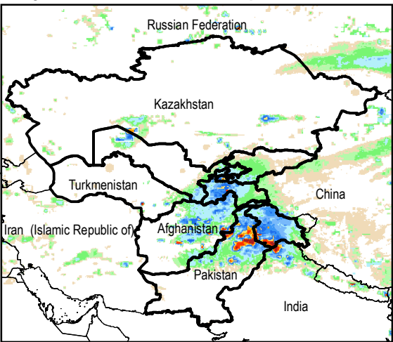
Daily Rainfall estimate for 1 Apr., 2015
