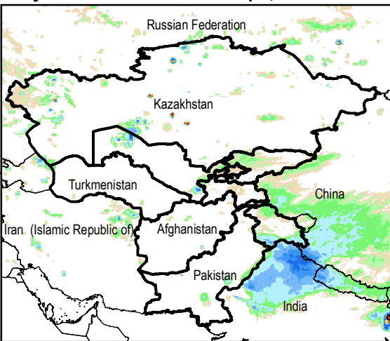
Daily Rainfall estimate for 7 Apr., 2015
