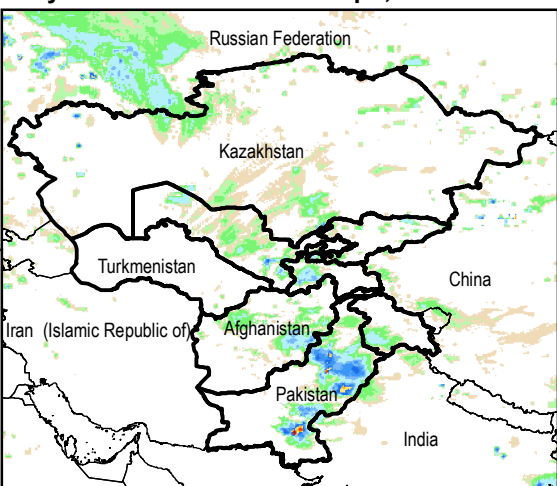
Daily Rainfall estimate for 6 Apr., 2015
