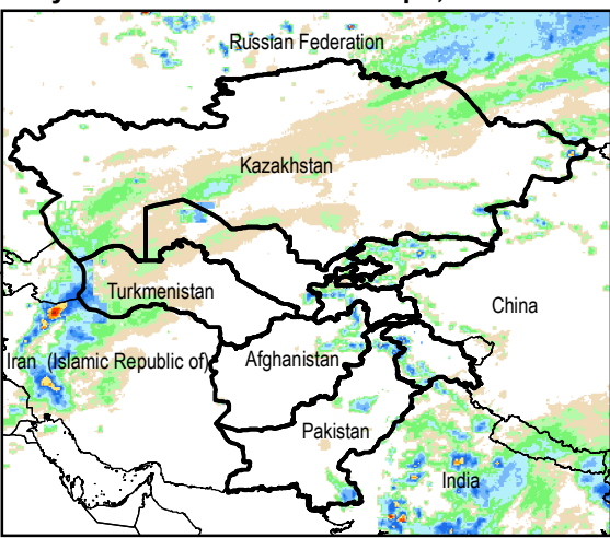
Daily Rainfall estimate for 12 Apr., 2015
