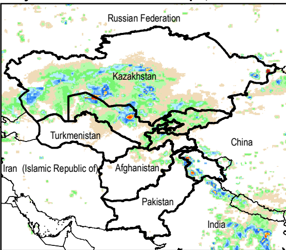
Daily Rainfall estimate for 17 Apr., 2015
