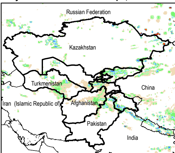
Daily Rainfall estimate for 29 Apr., 2015
