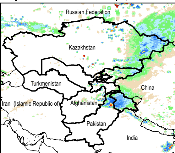
Daily Rainfall estimate for 27 Apr., 2015
