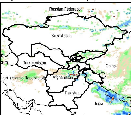
Daily Rainfall estimate for 28 Apr., 2015
