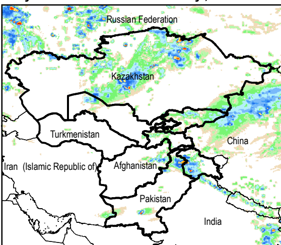
Daily Rainfall estimate for 18 May., 2015
