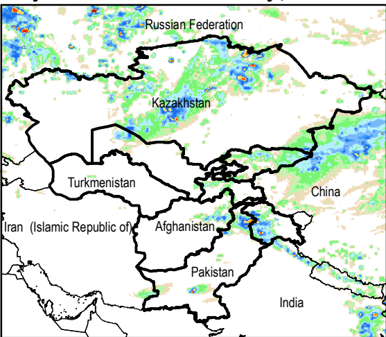
Daily Rainfall estimate for 21 May., 2015
