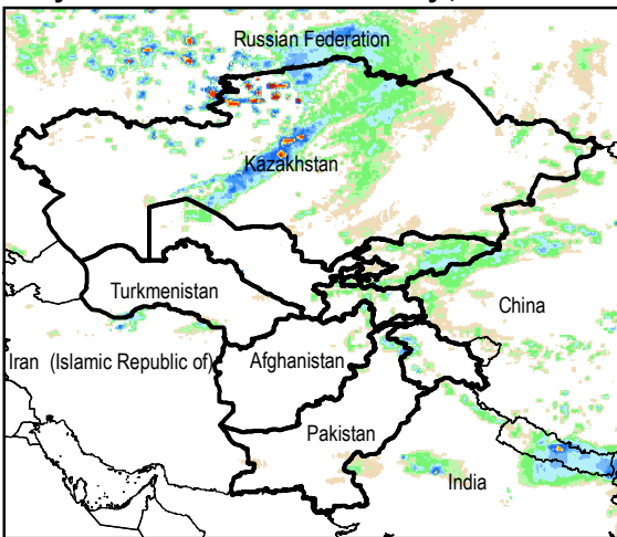
Daily Rainfall estimate for 23 May., 2015
