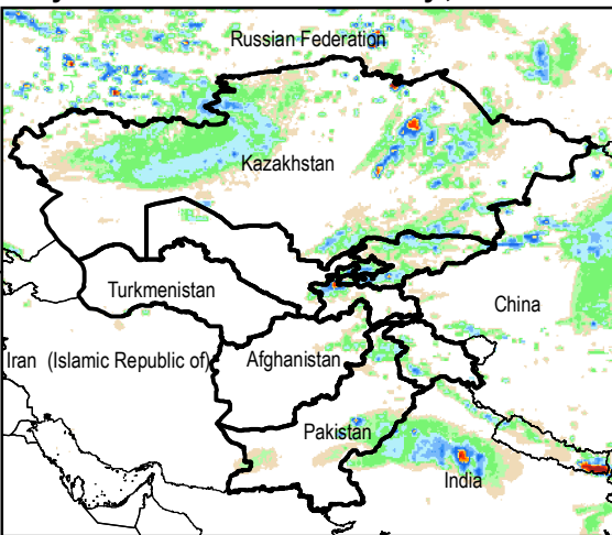
Daily Rainfall estimate for 22 May., 2015
