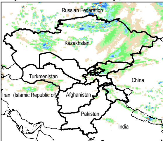
Daily Rainfall estimate for 24 May., 2015
