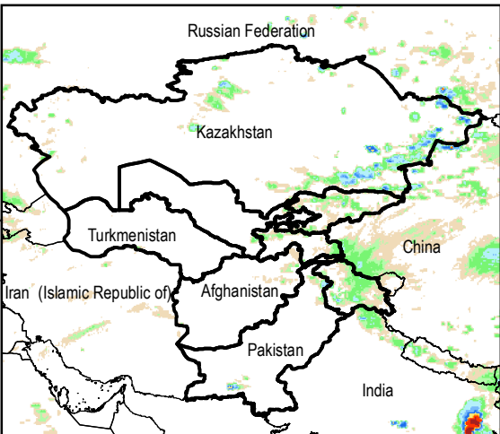
Daily Rainfall estimate for 26 May., 2015
