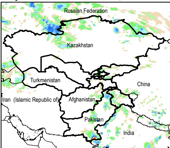
Daily Rainfall estimate for 6 Jun., 2015
