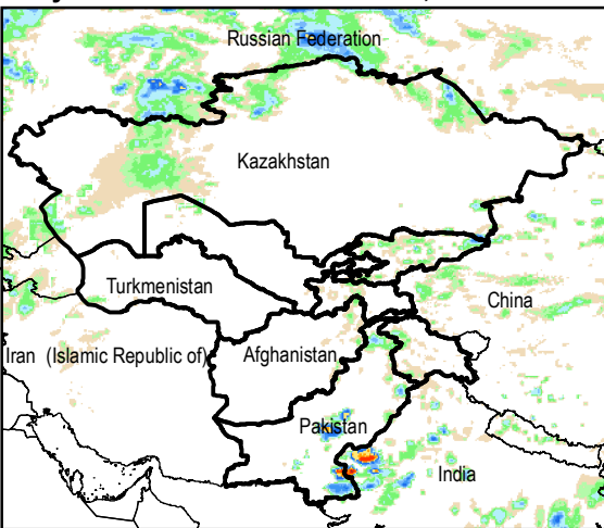
Daily Rainfall estimate for 5 Jun., 2015
