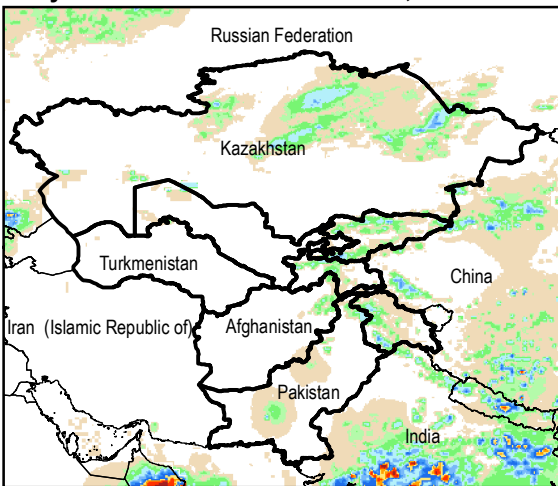
Daily Rainfall estimate for 15 Jun., 2015
