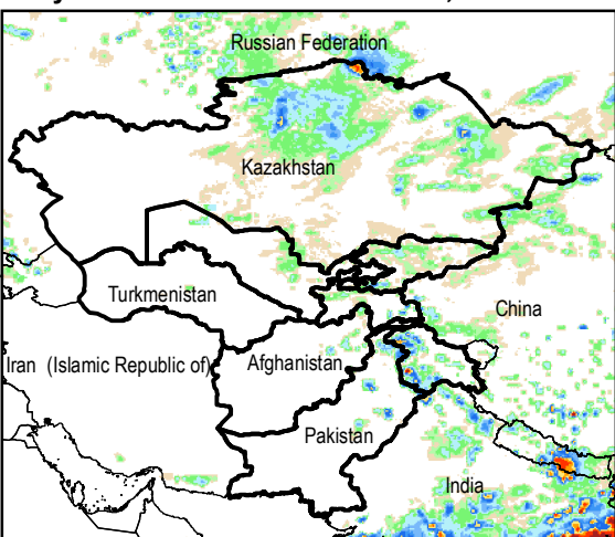
Daily Rainfall estimate for 13 Jun., 2015
