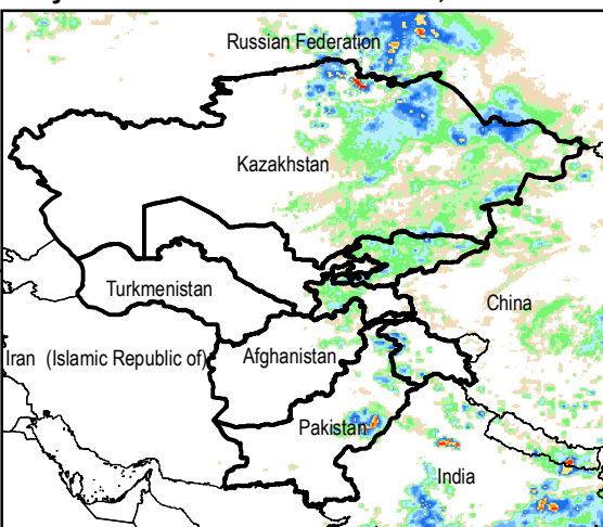
Daily Rainfall estimate for 14 Jun., 2015
