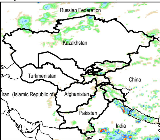
Daily Rainfall estimate for 22 Jun., 2015
