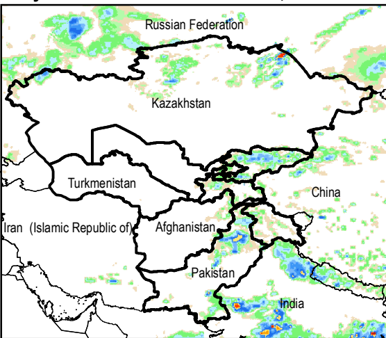
Daily Rainfall estimate for 23 Jun., 2015
