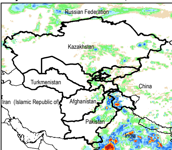
Daily Rainfall estimate for 24 Jun., 2015
