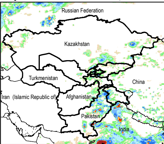
Daily Rainfall estimate for 26 Jun., 2015
