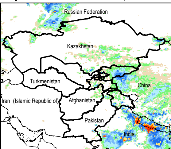
Daily Rainfall estimate for 25 Jun., 2015
