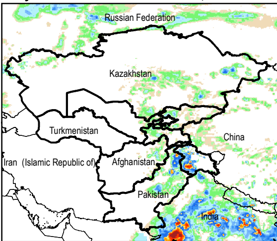
Daily Rainfall estimate for 27 Jun., 2015
