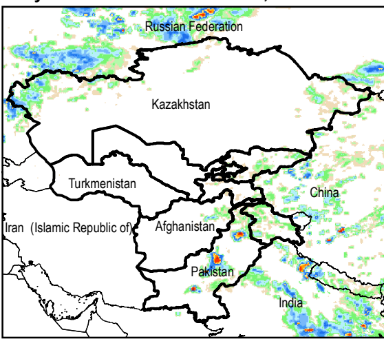
Daily Rainfall estimate for 1 Jul., 2015
