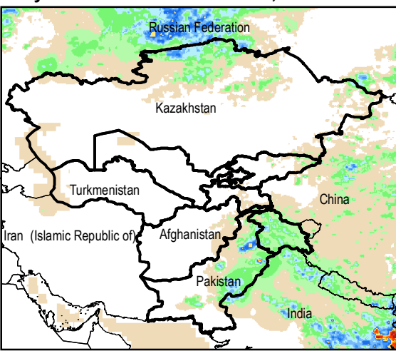
Daily Rainfall estimate for 2 Jul., 2015
