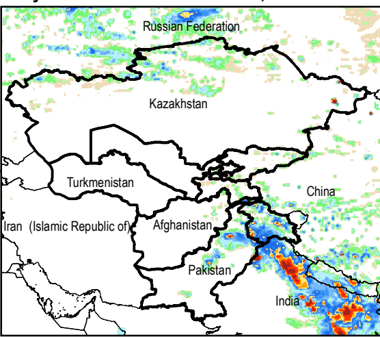
Daily Rainfall estimate for 6 Jul., 2015
