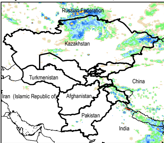
Daily Rainfall estimate for 7 Jul., 2015
