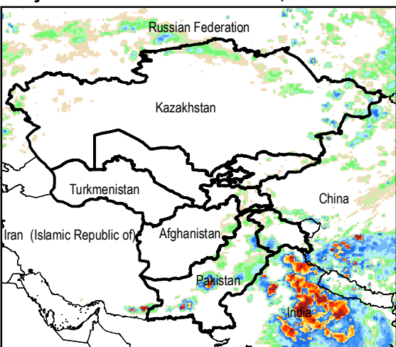
Daily Rainfall estimate for 11 Jul., 2015
