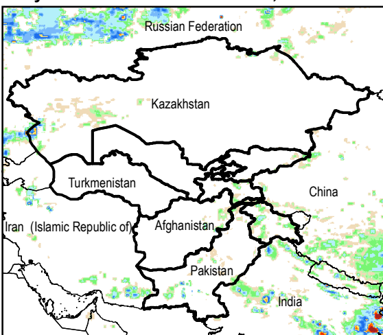
Daily Rainfall estimate for 13 Jul., 2015
