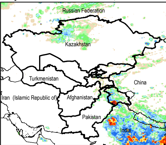
Daily Rainfall estimate for 12 Jul., 2015
