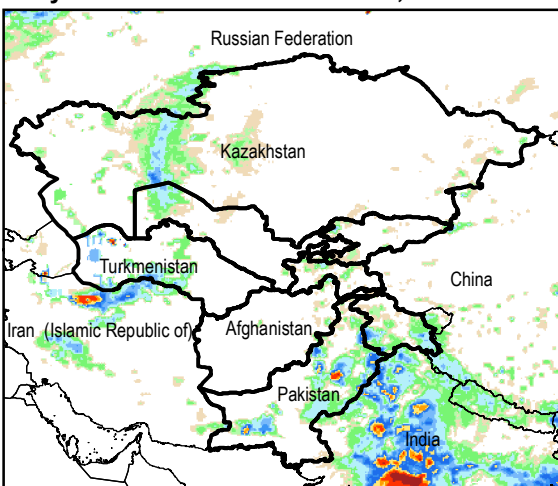
Daily Rainfall estimate for 20 Jul., 2015
