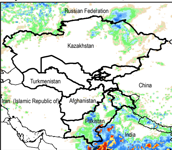
Daily Rainfall estimate for 25 Jul., 2015
