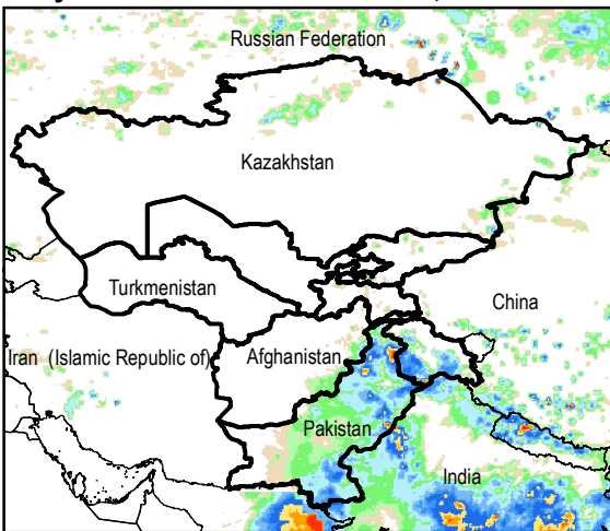
Daily Rainfall estimate for 26 Jul., 2015
