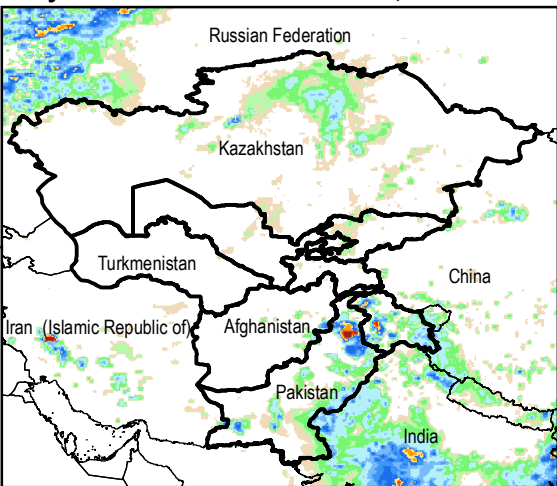
Daily Rainfall estimate for 24 Jul., 2015
