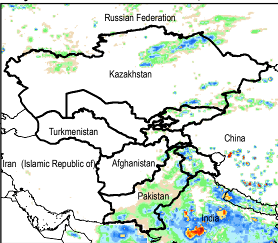
Daily Rainfall estimate for 27 Jul., 2015
