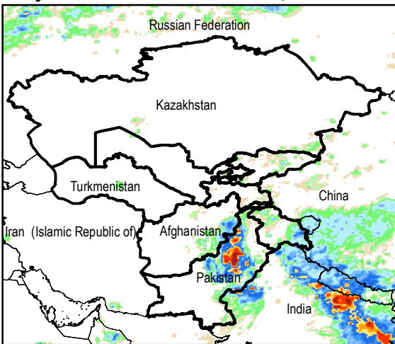
Daily Rainfall estimate for 3 Aug., 2015
