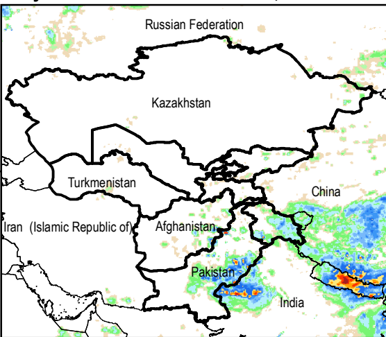
Daily Rainfall estimate for 2 Aug., 2015
