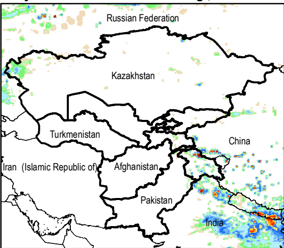
Daily Rainfall estimate for 22 Aug., 2015
