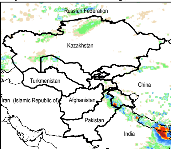
Daily Rainfall estimate for 23 Aug., 2015
