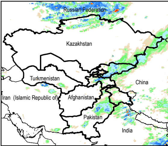
Daily Rainfall estimate for 26 Aug., 2015
