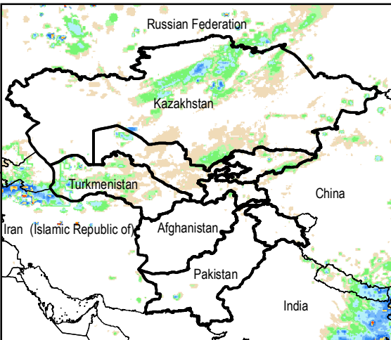
Daily Rainfall estimate for 25 Aug., 2015
