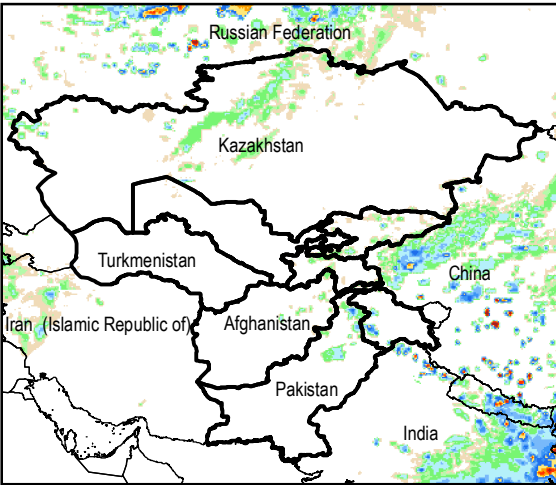
Daily Rainfall estimate for 3 Sep., 2015
