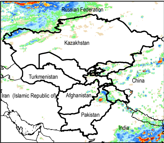
Daily Rainfall estimate for 2 Sep., 2015
