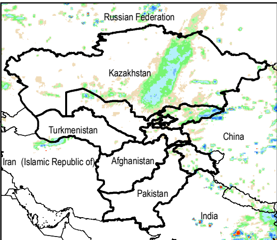
Daily Rainfall estimate for 2 Sep., 2015
