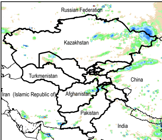
Daily Rainfall estimate for 4 Sep., 2015
