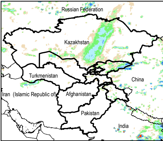
Daily Rainfall estimate for 5 Sep., 2015
