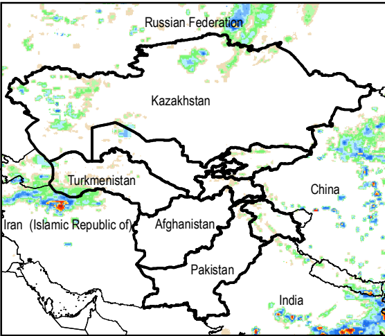
Daily Rainfall estimate for 4 Sep., 2015
