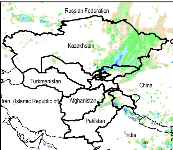
Daily Rainfall estimate for 3 Sep., 2015
