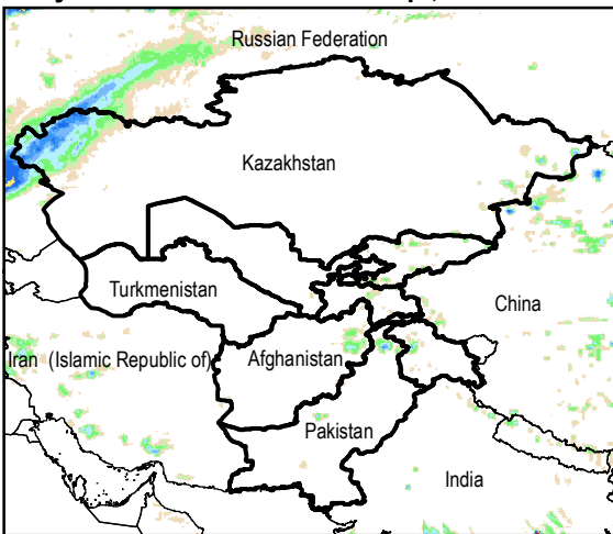
Daily Rainfall estimate for 12 Sep., 2015
