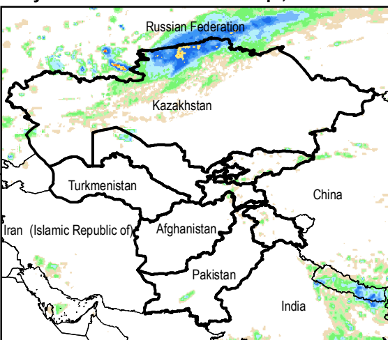
Daily Rainfall estimate for 11 Sep., 2015
