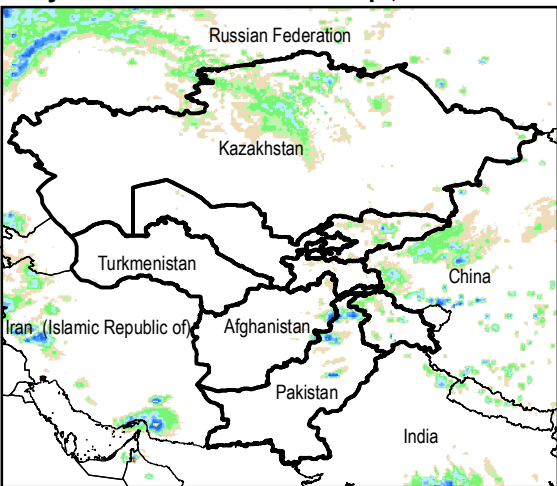
Daily Rainfall estimate for 10 Sep., 2015
