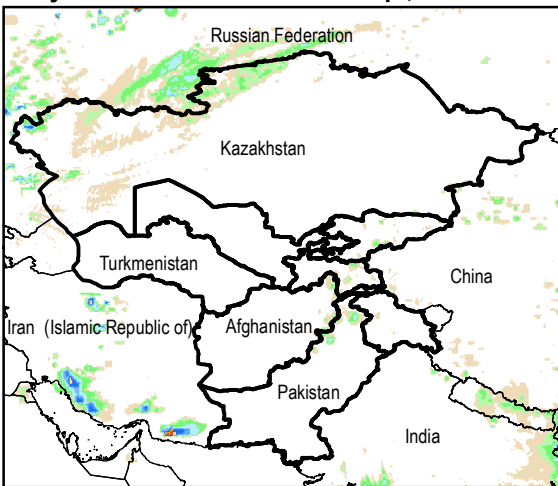
Daily Rainfall estimate for 13 Sep., 2015
