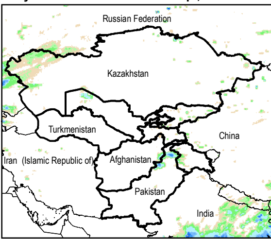
Daily Rainfall estimate for 15 Sep., 2015
