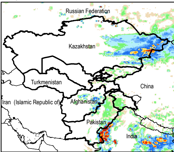
Daily Rainfall estimate for 21 Sep., 2015
