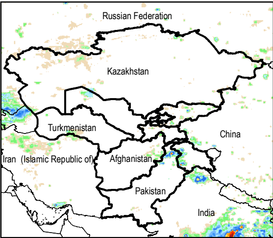
Daily Rainfall estimate for 19 Sep., 2015
