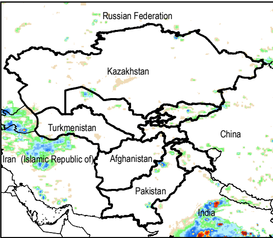
Daily Rainfall estimate for 20 Sep., 2015
