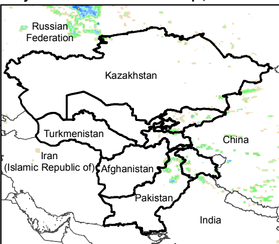
Daily Rainfall estimate for 26 Sep., 2015
