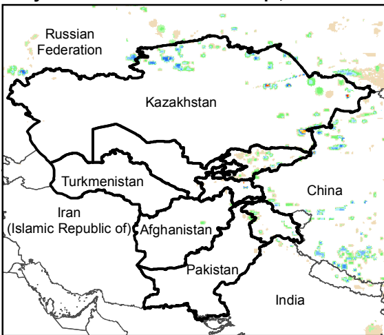
Daily Rainfall estimate for 27 Sep., 2015
