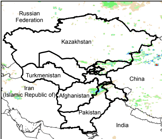
Daily Rainfall estimate for 28 Sep., 2015
