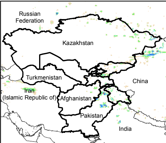
Daily Rainfall estimate for 27 Sep., 2015
