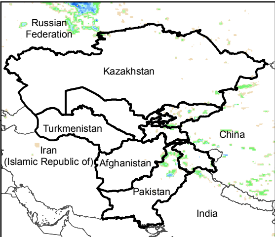
Daily Rainfall estimate for 26 Sep., 2015
