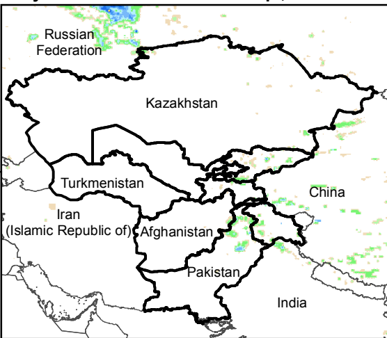
Daily Rainfall estimate for 29 Sep., 2015
