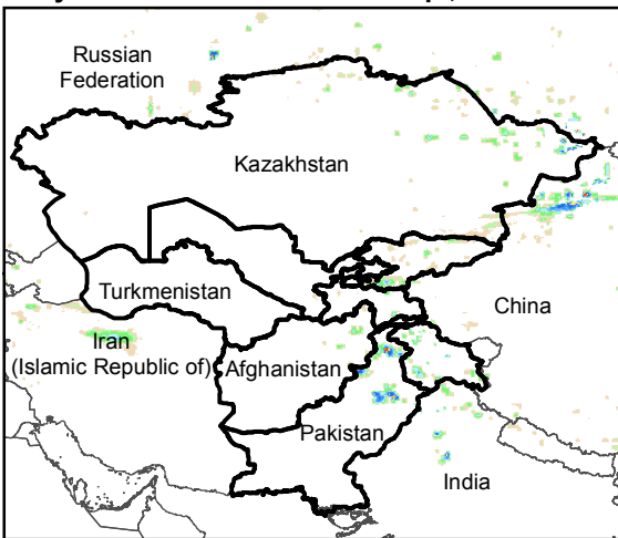
Daily Rainfall estimate for 30 Sep., 2015
