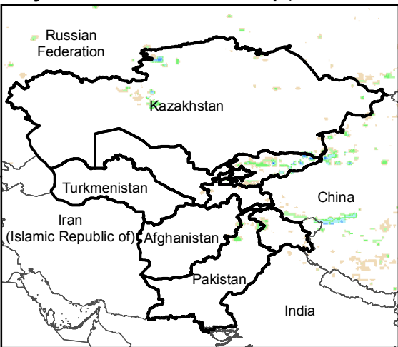
Daily Rainfall estimate for 28 Sep., 2015
