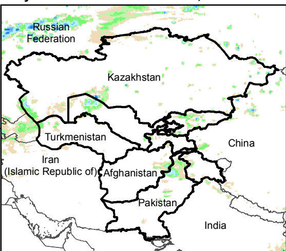
Daily Rainfall estimate for 6 Oct., 2015
