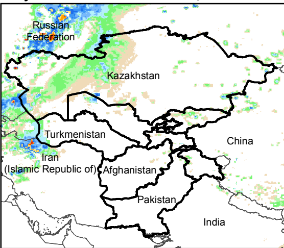
Daily Rainfall estimate for 11 Oct., 2015
