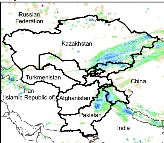
Daily Rainfall estimate for 17 Oct., 2015
