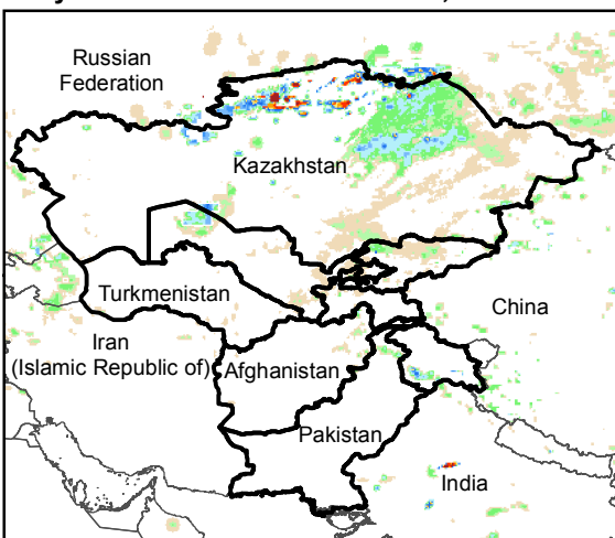
Daily Rainfall estimate for 21 Oct., 2015
