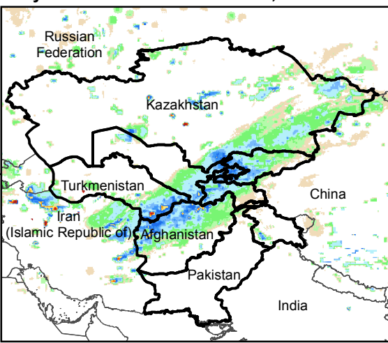
Daily Rainfall estimate for 1 Nov., 2015
