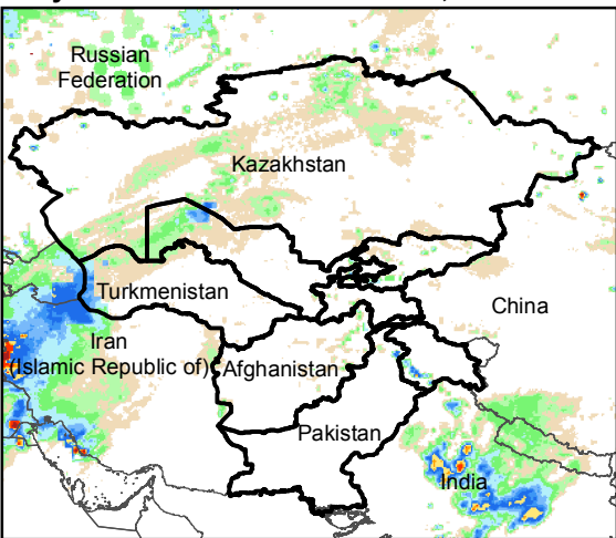
Daily Rainfall estimate for 31 Oct., 2015
