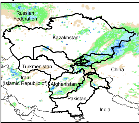
Daily Rainfall estimate for 2 Nov., 2015
