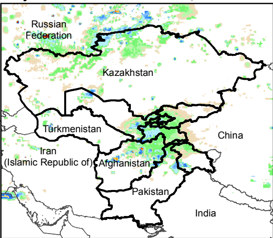
Daily Rainfall estimate for 6 Nov., 2015
