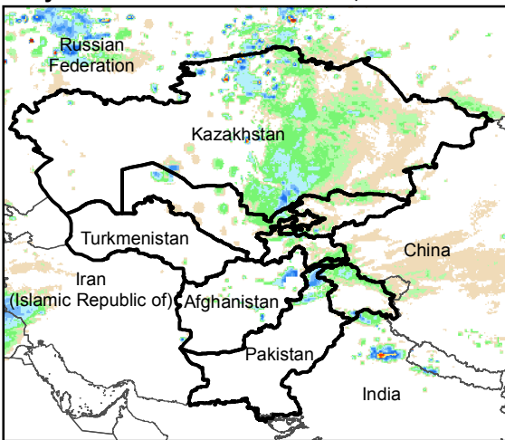
Daily Rainfall estimate for 8 Nov., 2015
