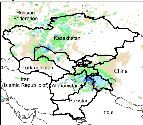
Daily Rainfall estimate for 7 Nov., 2015
