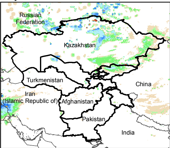
Daily Rainfall estimate for 9 Nov., 2015
