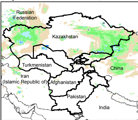
Daily Rainfall estimate for 19 Nov., 2015
