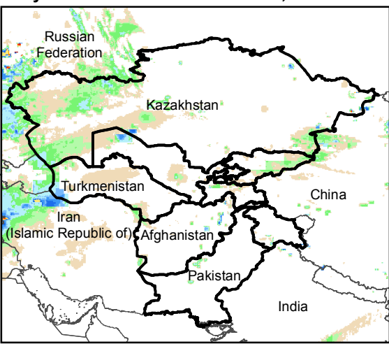
Daily Rainfall estimate for 17 Nov., 2015
