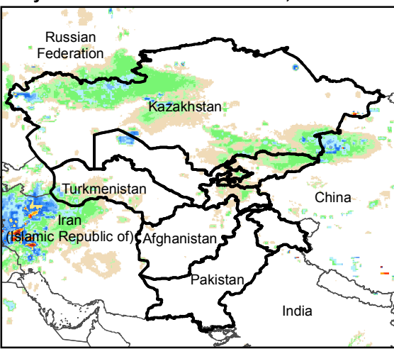
Daily Rainfall estimate for 18 Nov., 2015
