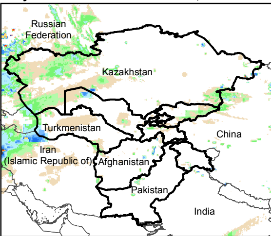
Daily Rainfall estimate for 20 Nov., 2015
